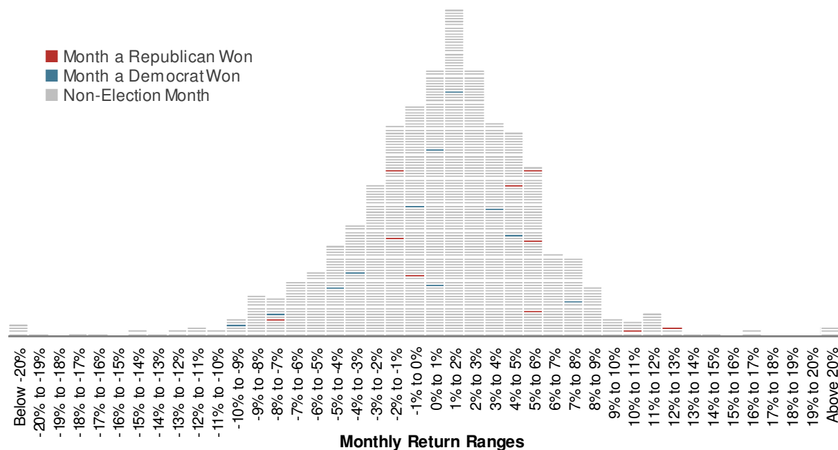
Exhibit 1. Presidential Elections and S&P 500 Returns Histogram of Monthly Returns, January 1926–June 2016
